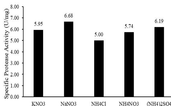
Figure 3. Effects of different nitrogen sources on protease production by PUA-14 bacterial isolate
