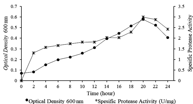
Figure 1. Growth profile and specific protease activity of PUA-14 bacterial isolates
