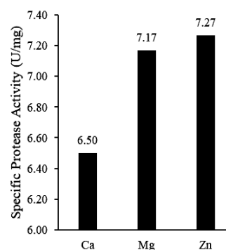
Figure 4. Effects of different trace elements on protease production by PUA-14 bacterial isolate
