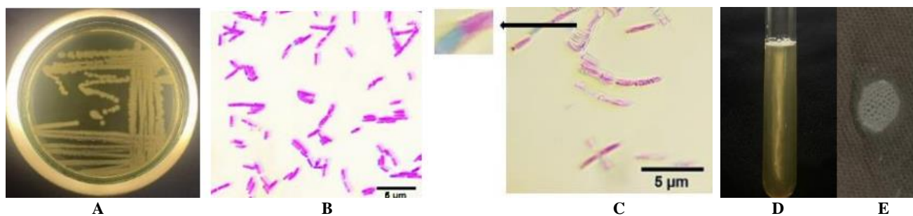
Figure 6. A. Macroscopic observation of PUA-14 bacterial isolates; B. Gram staining; C. Endospore staining; D. Motility test; E. Catalase test
