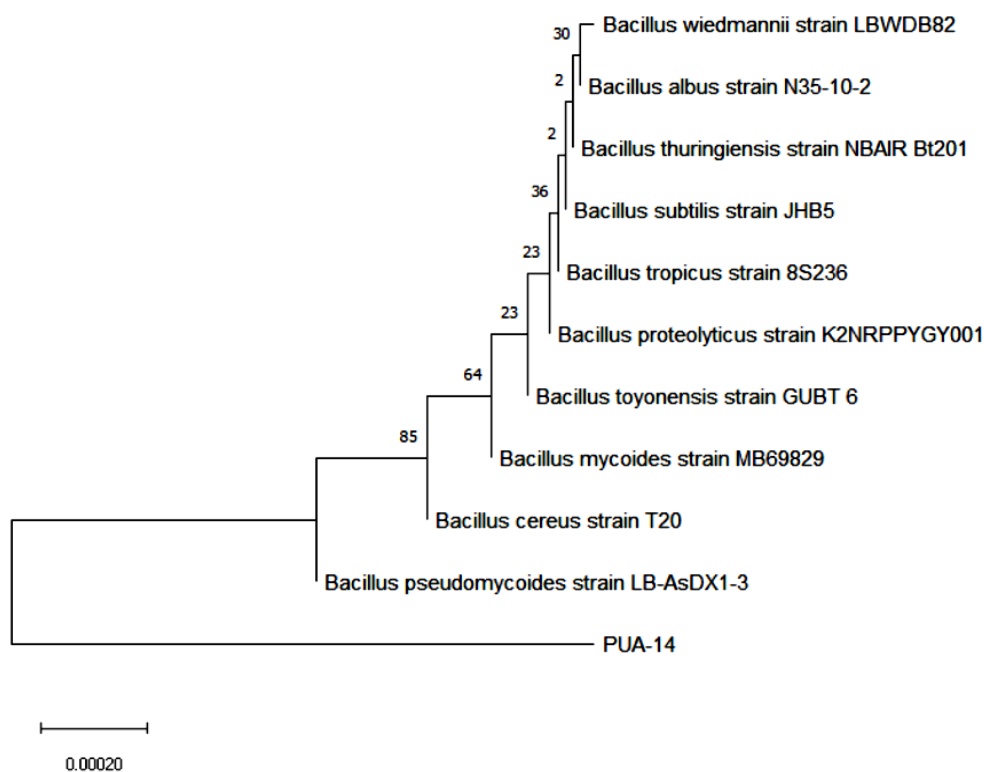
Figure 7. Phylogenetic tree of PUA-14 bacterial isolates using Neighbor-Joining (NJ) analysis based on 16S rRNA sequences
