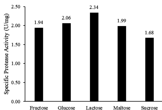
Figure 2. Effects of different carbon sources on protease production by PUA-14 bacterial isolate
