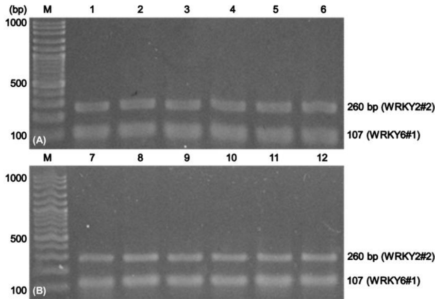
Figure 5. Primer concentration affects SNAP marker amplification of coconut in duplex PCR. Amplicons yielded from duplex PCR using primer concentration of either (A) 0.75 \mu L of 10 \mu M or (B) 0.375 \mu L of 10 \mu M for each primer. For each duplex PCR reaction, two primer pairs consisting of WRKY6#1 Ref and WRKY2#2 Alt were used to amplify two different amplicon sizes. Duplex PCR amplification of DNA template using both WRKY6#1 and WRKY2#2 primer pairs was done using T_a=55.4^\circ\text{C} , and the expected amplicon size was either 107 bp or 260 bp, respectively. All tested primers were used with their appropriate reverse primers while the PCR reactions were done using the same Kalianda Tall Kopyor coconut DNA template
