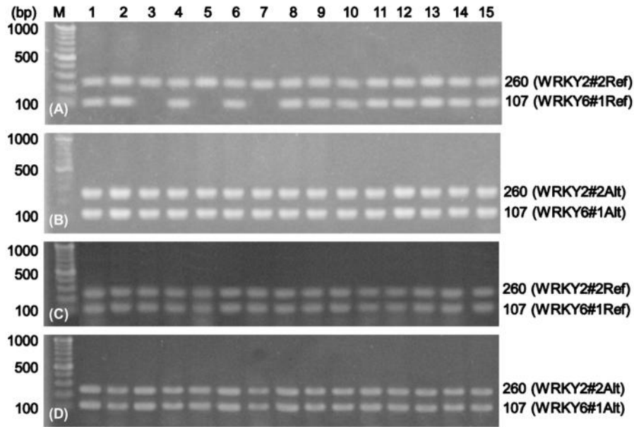
Figure 7. Representative results of SNAP marker application to genotype Pati Dwarf (A and B) and Jember Tall (C and D) Kopyor coconut using duplex PCR. The genotyping was conducted using two pairs of WRKY specific SNAP markers in a duplex PCR reaction. The two primer pairs are WRKY6#1Ref and WRKY2#2Ref (A and C) and WRKY6#1Alt and WRKY2#2Alt (B and D). We used all of those primers in duplex PCR with their appropriate reverse primers. 1-15, 15 samples of either Pati Dwarf or Jember Tall Kopyor coconuts. M, a size control of 100 bp DNA ladder
