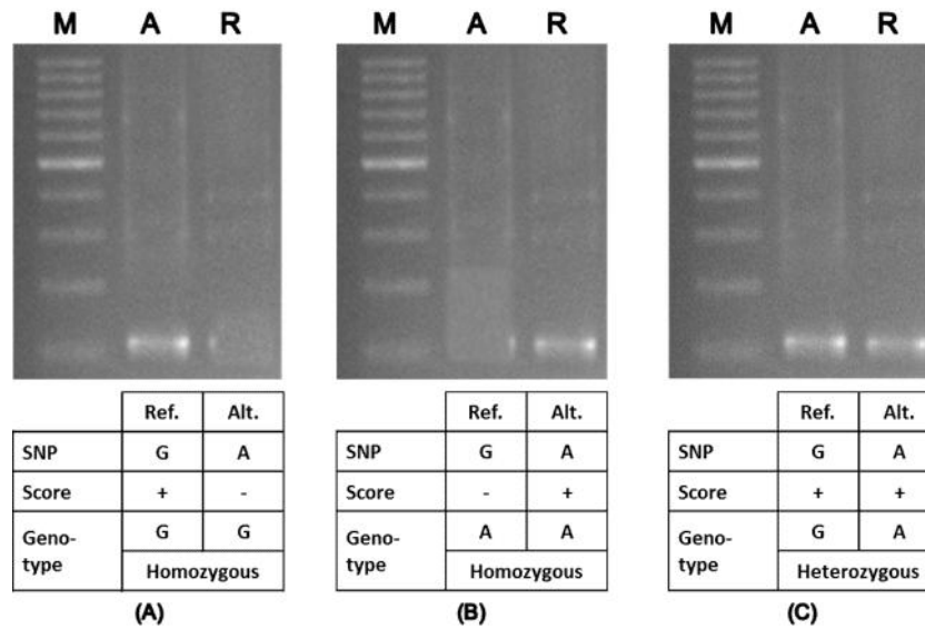
Figure 3. Genotyping of coconut with SNAP markers using singleplex PCR results in three possible coconut genotypes. (A) Homozygous for Ref, it scores (+) for Ref and (-) for Alt. The genotypes for the plant is GG, (B) homozygous for Alt, its scores (-) for Ref and (+) for Alt. The genotypes for the plant is AA and (C) heterozygous for Ref and Alt, its score (+) for Ref and (+) for Alt. The genotype of the plant is AG
