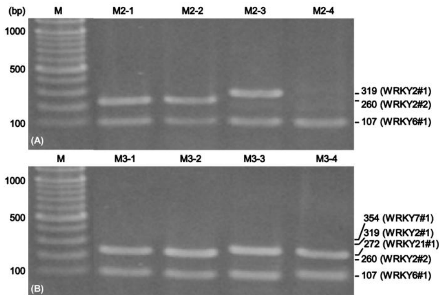
Figure 6. Multiplex PCR to amplify SNAP marker from coconut using (A) duplex PCR and (B) triplex PCR. For each duplex PCR reaction, the primer pairs used for M2-1 were WRKY6#1 Ref and WRKY2#2 Ref while for M2-2-WRKY6#1 Alt and WRKY2#2 Alt; for M2-3 were WRKY6#1 Ref and WRKY2#1 Ref while for M2-4-WRKY6#1 Alt and WRKY2#1 Alt. For each triplex PCR, the primer pairs used for M3-1 were WRKY6#1 Ref, WRKY2#2 Ref, and WRKY21#1 Ref while M3-2-WRKY6#1 Alt, WRKY2#2 Alt and WRKY21#1 Alt; for M3-3 were WRKY6#1 Ref, WRKY21#1 Ref, and WRKY7#1 Ref while M3-4-WRKY6#1 Alt, WRKY21#1 Alt and WRKY7#1 Alt. The T_a was set at 55.4^\circ\text{C} (M2-1, M2-2, M3.1, and M3.2); 48.8^\circ\text{C} (M2-3 and M2-4) or 52.6^\circ\text{C} (M3.3 and M3.4). All primers were used with their appropriate reverse primer while the PCR reactions were done using the same Pati Dwarf Kopyor coconut DNA template
