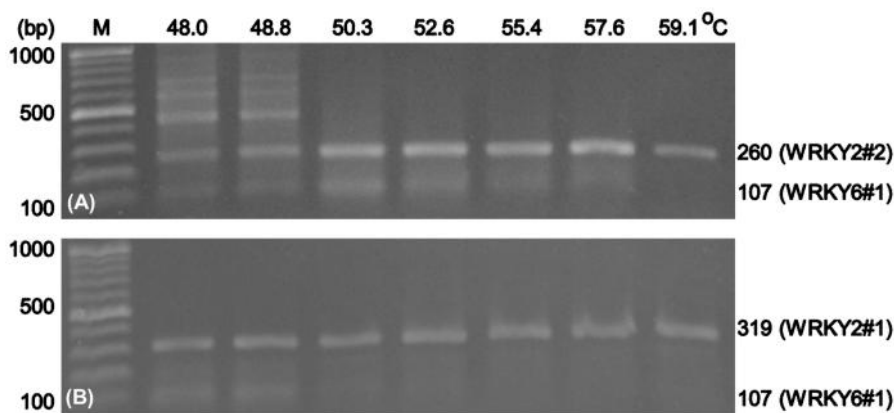
Figure 4. Annealing temperature affects SNAP marker amplification of coconut in duplex PCR. We evaluated effects of annealing temperatures in duplex PCR and each PCR reaction. The two primer pairs consisted of (A) WRKY6#1 Ref and WRKY2#2 Alt or (B) WRKY6#1 Alt and WRKY2#1 Ref-were used to amplify two different sizes of amplicons. Amplification of DNA template using WRKY6#1, both Ref and Alt yielded 107 bp, WRKY2#1-319 bp and WRKY2#2-260 bp amplicons, respectively. All tested primers were used with their appropriate reverse primers while the PCR reactions were done using the same Kalianda Tall Kopyor coconut DNA template
