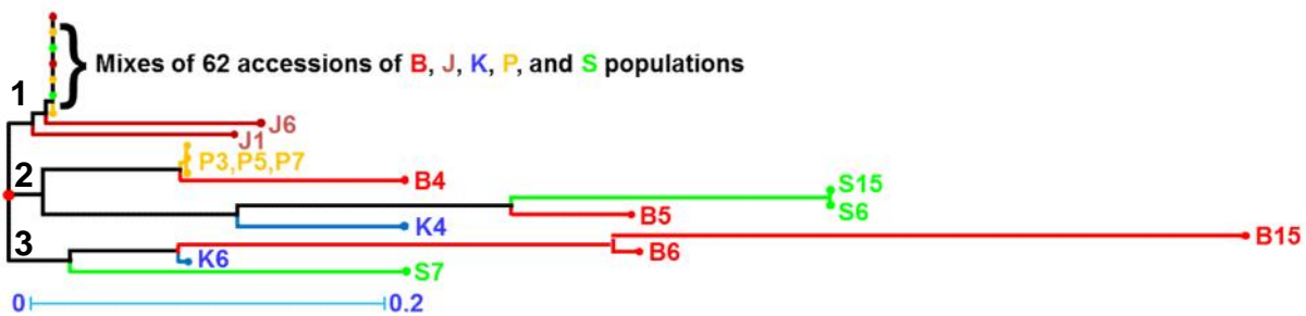
Figure 8. Unrooted Neighbour-Joining tree (weighted) realized based on dissimilarity matrix for Banten Tall (B), Jember Tall (J), Kalianda Tall (K), Pati Dwarf (P), and Sumenep Tall (S) Kopyor coconuts based on four loci of SNAP marker genotype data. The SNAP markers were generated using duplex PCR. The tree shows a total of 75 individuals (15 individuals per population) of B, J, K, P and S Kopyor coconuts
