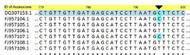
Figure 1. An example of multiple sequence alignment results over seven accessions of WRKY6 DNA fragments and the identified bi-allelic single nucleotide polymorphism (SNP) site #3 at the base position of 795. The bi-allelic nucleotide variants are either T (57.1%) or C (42.9%).
