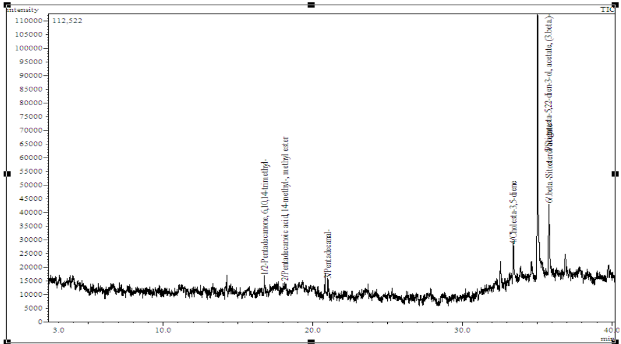
Figure S9. Chromatogram of hexane extracts of Cymodocea serrulata leaves
