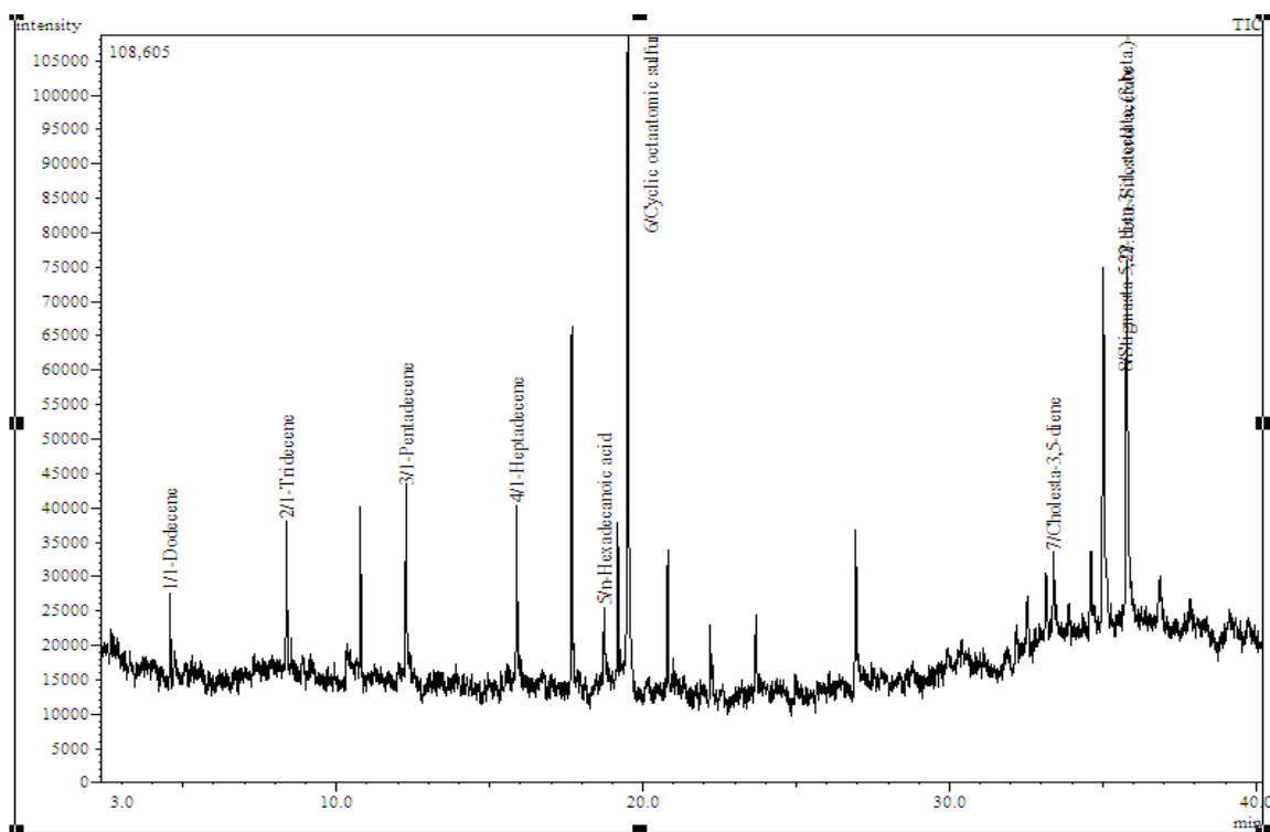
Figure S4. Chromatogram of hexane extracts of Thalassia hemprichii roots
