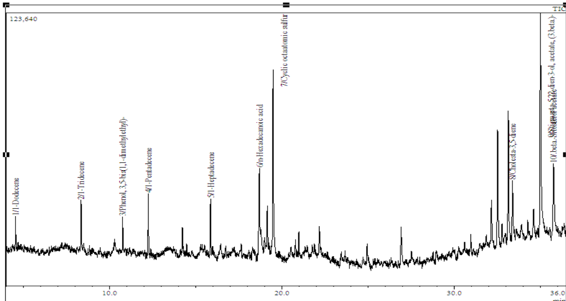
Figure S3. Chromatogram of hexane extracts of Thalassia hemprichii leaves
