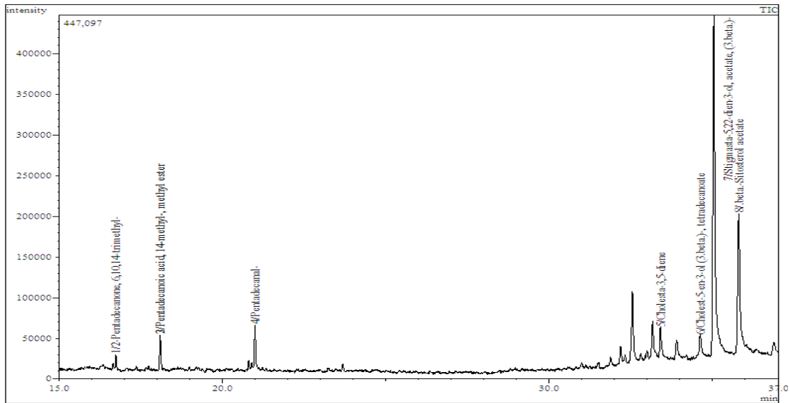
Figure S1. Chromatogram of hexane extracts of Cymodocea rotundata leaves
