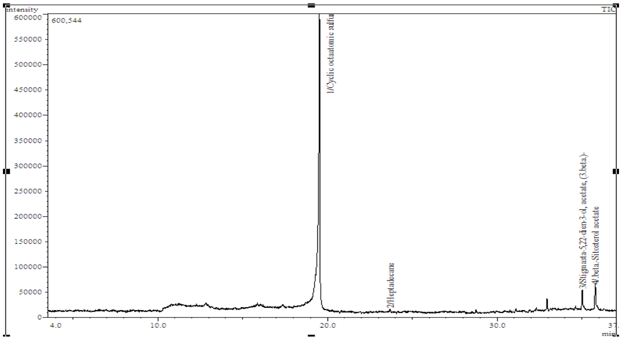
Figure S11. Chromatogram of hexane extracts of Enhalus acoroides roots
