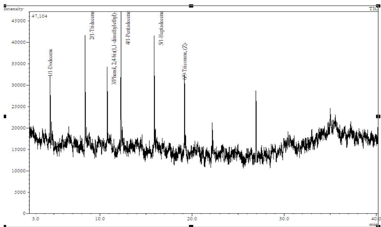
Figure S8. Chromatogram of hexane extracts of Syringodium isoetifolium roots
