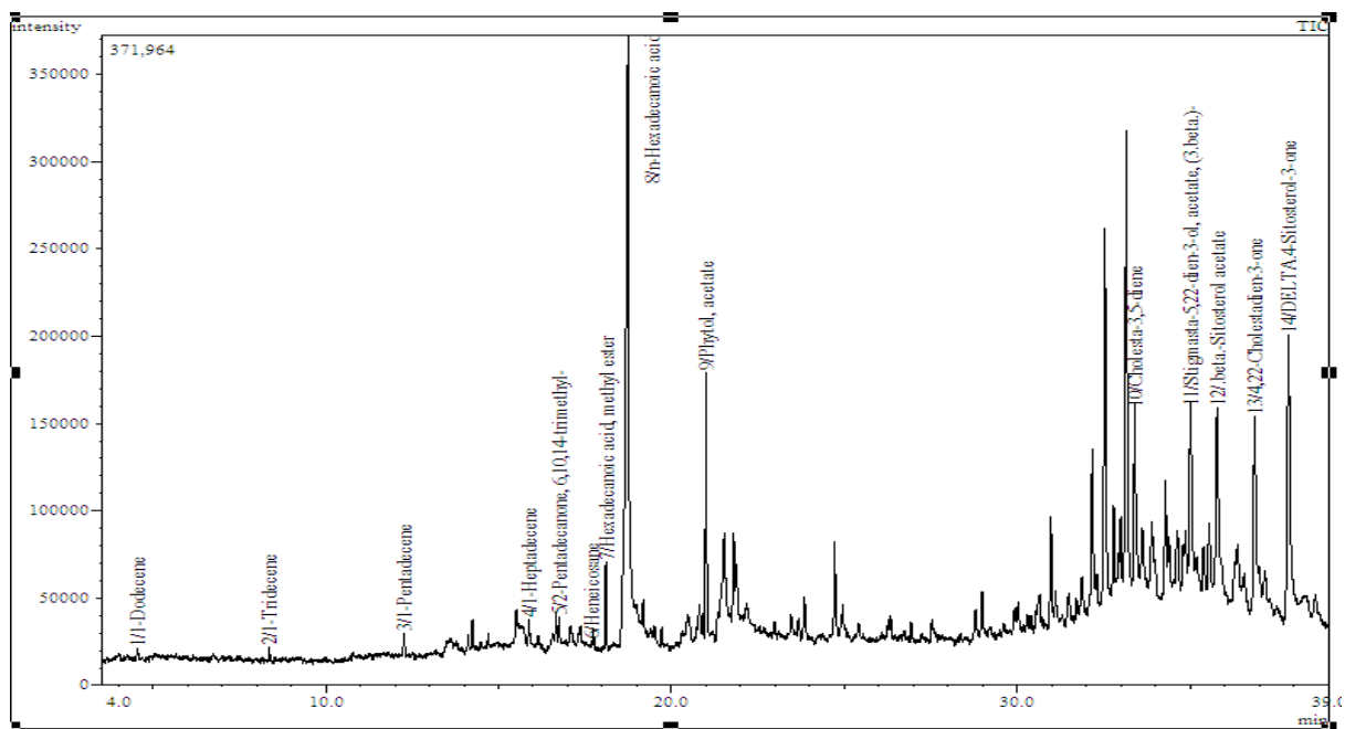
Figure S12. Chromatogram of hexane extracts of Halodule uninervis roots
