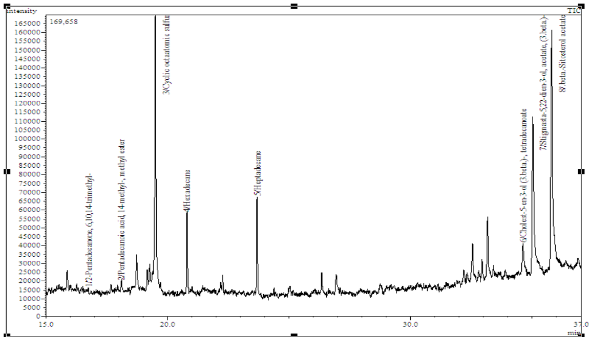
Figure S2. Chromatogram of hexane extracts of Cymodocea rotundata roots
