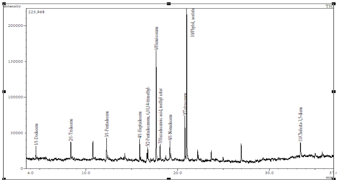
Figure S5. Chromatogram of hexane extracts of Thalassodendron ciliatum leaves
